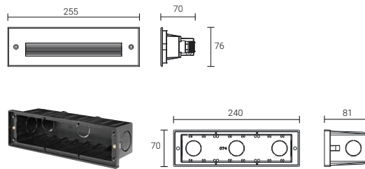
Mounting sleeve 074#
