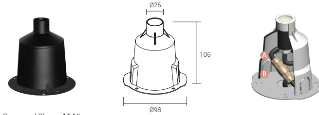
Recessed Sleeve 114#
