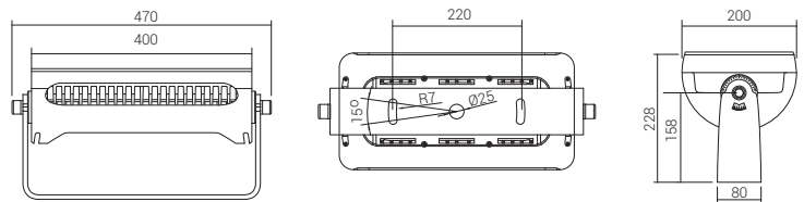
MS3HMA1278UD/C/R/F (u-shaped bracket)
