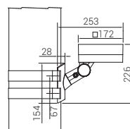
MS3HMX1236H (tree bracket)
