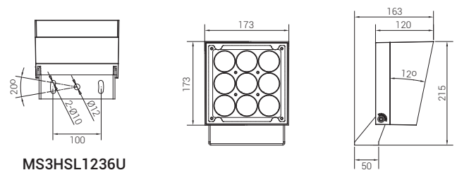
MS3HSL1236U (u-shaped bracket)
