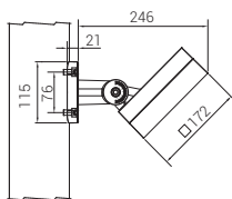
MS3HMX1236L (pole mounted screw fixed part)
