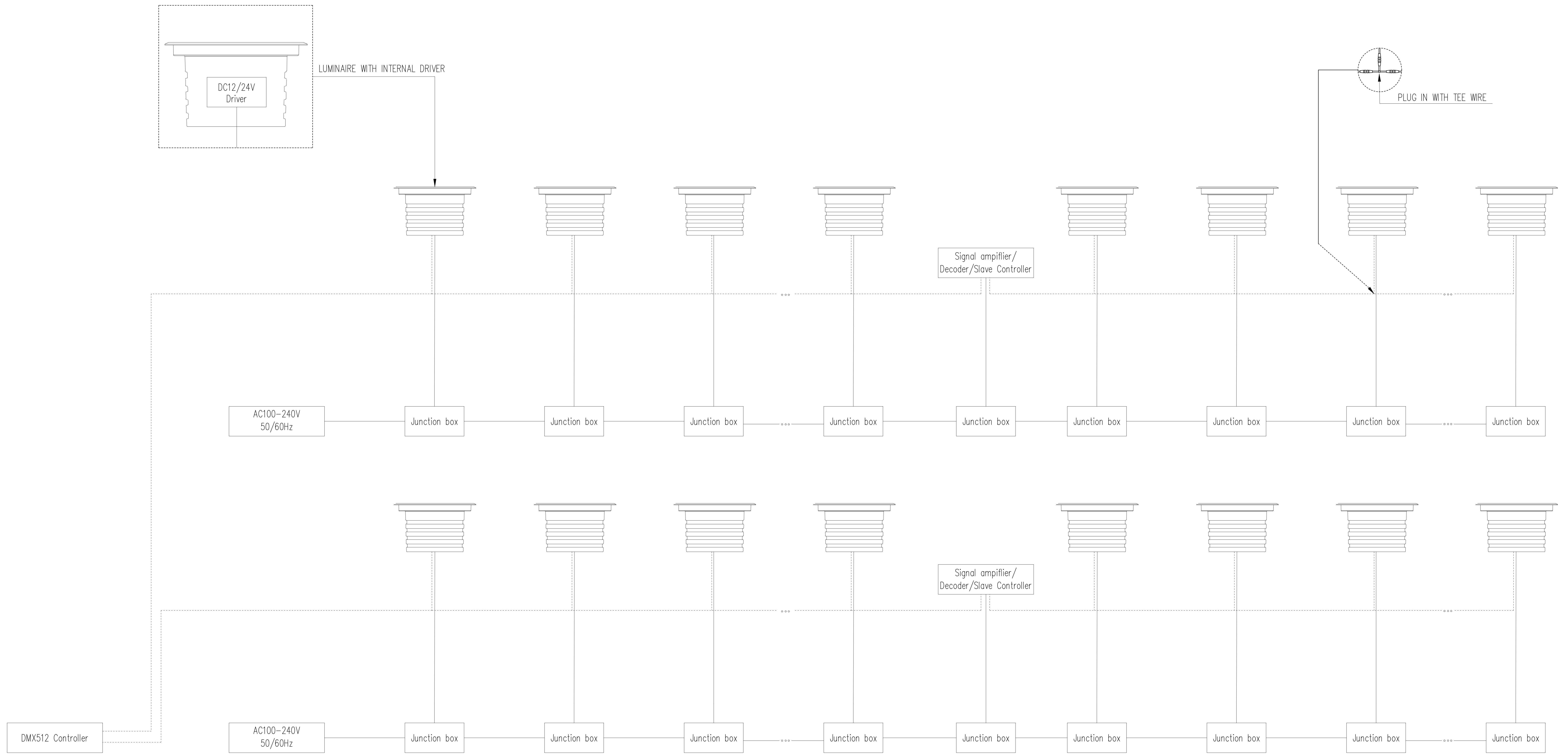
DMX RGB/RGBW TYPE 2 WIRING DIAGRAM INTERNAL DRIVER
