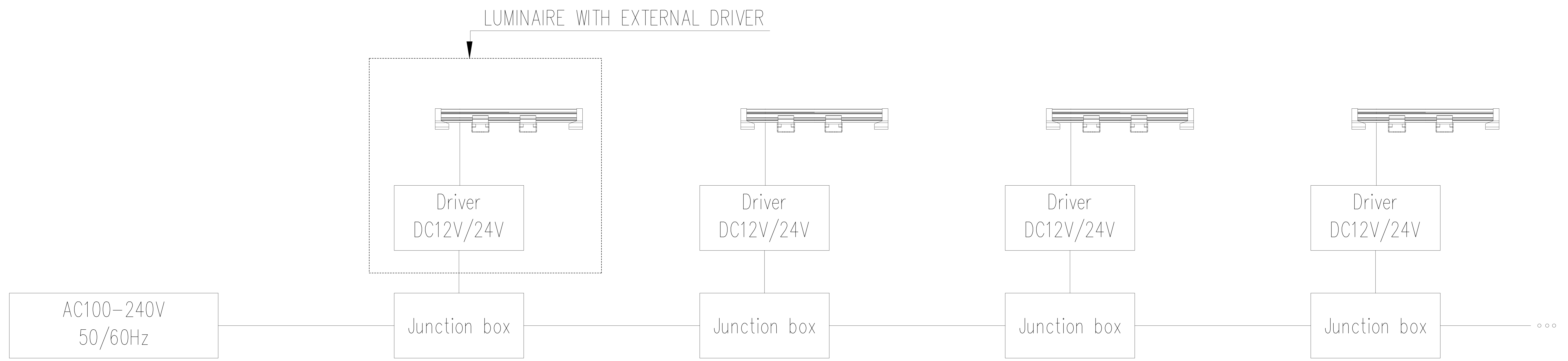
ON/OFF WIRING DIAGRAM - AN EXTERNAL DRIVER EACH LUMINAIRE
