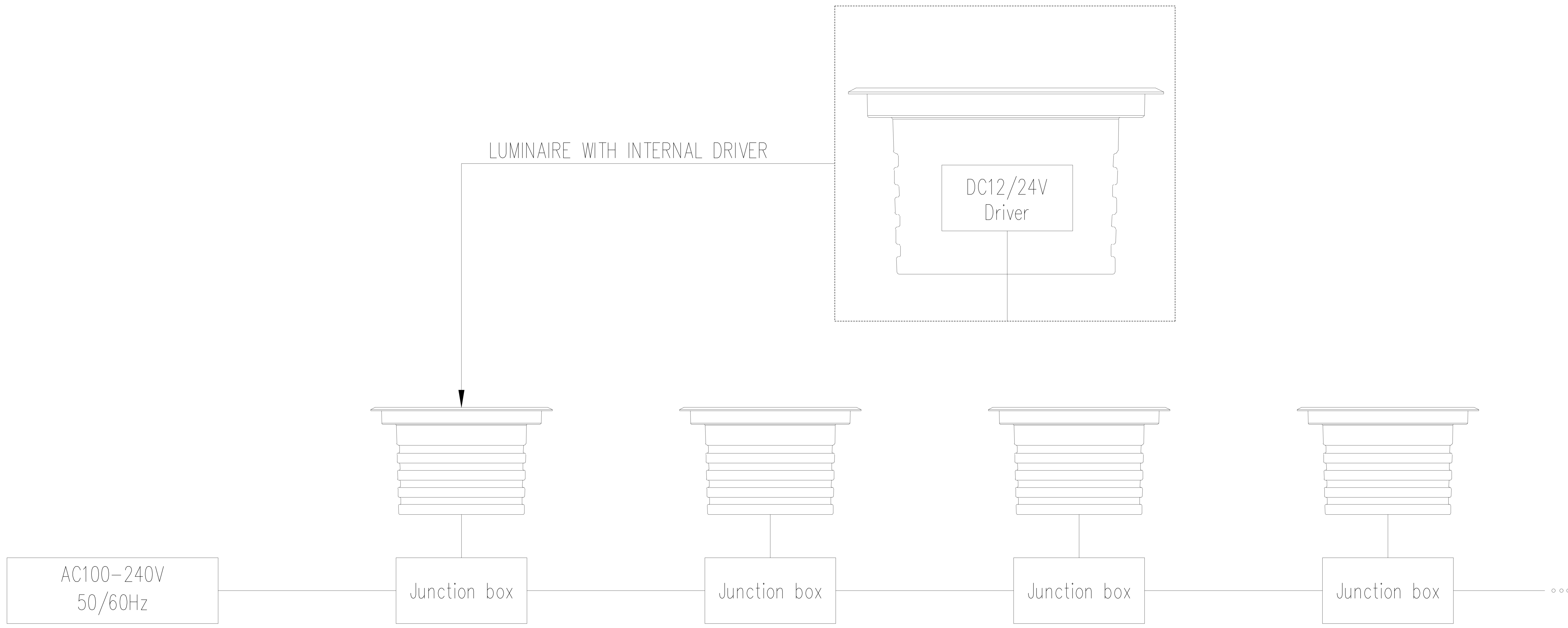
ON/OFF WIRING DIAGRAM - AN INTERNAL DRIVER EACH LUMINAIRE
