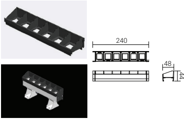
Anti-glare louver
