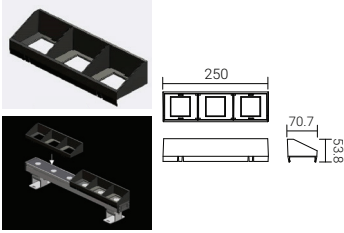
Anti-glare louver
