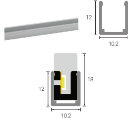
Aluminium profile
