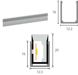
Aluminium profile
