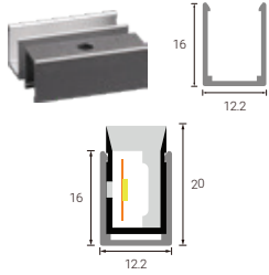
Mounting clips (aluminum)
