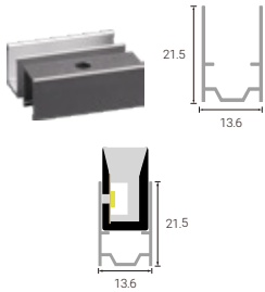
Mounting clips (aluminum)
