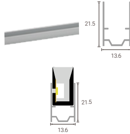
Aluminium profile
