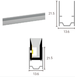
Aluminium profile
